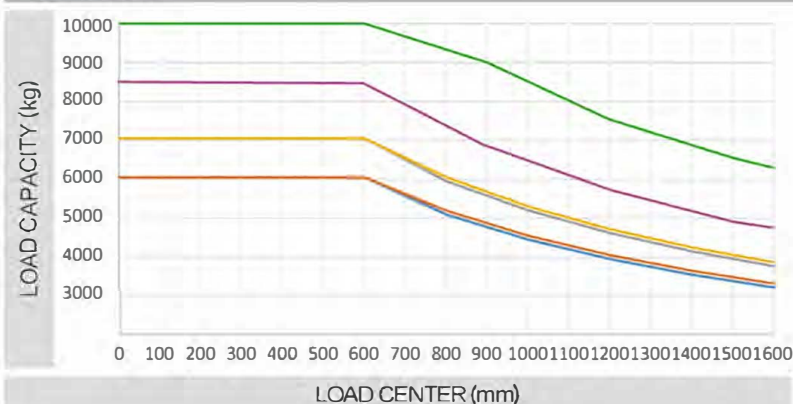
Load curve
